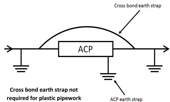
Fig1. Earth and Cross Bonding Schematic
